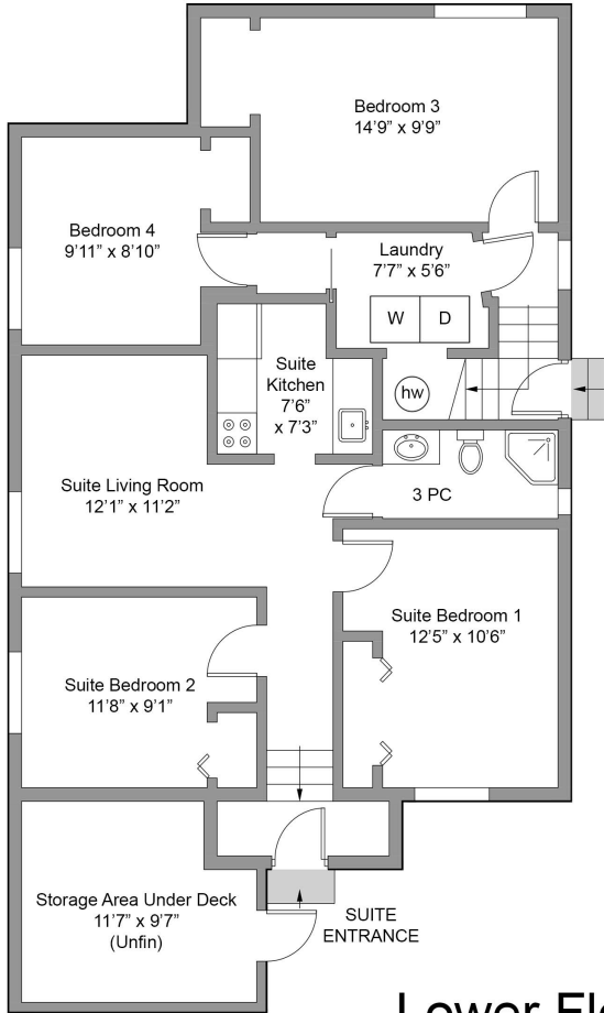
Lower Floor 1172 Sqft. (Avg Ht. - 7')
